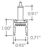
Straight Run
