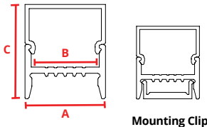
Mounting Clip
