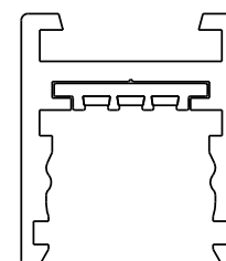
ST5-48/96/144-SF-XX Stenos Track, Surface
